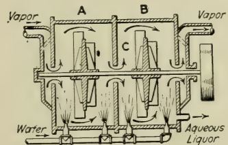
FIG. 66.—Reading Centrifugal Scrubber.
